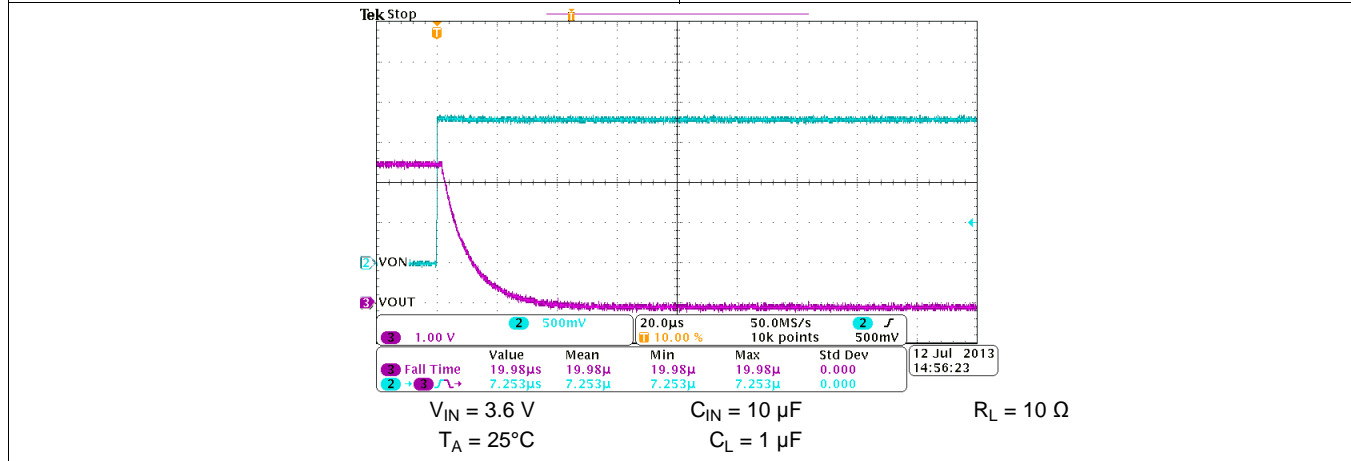
Figure 40. Turn-Off Response
