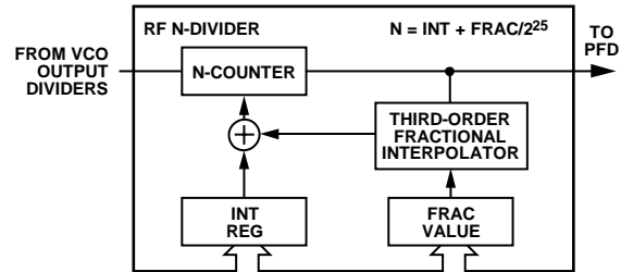
Figure 55. RF Fractional-N Divider
