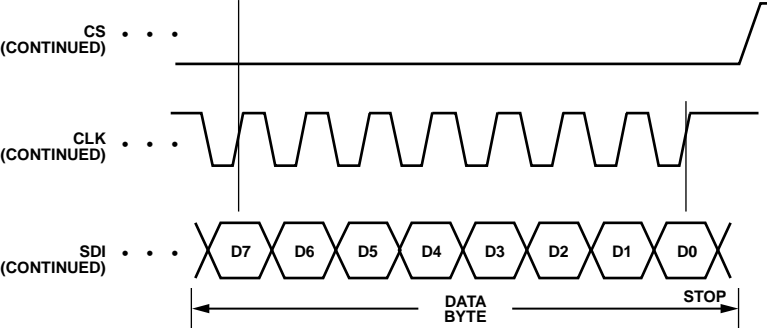
Figure 66. SPI Byte Write Example
