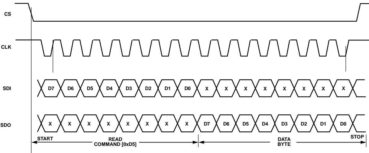
Figure 67. SPI Byte Read Example
