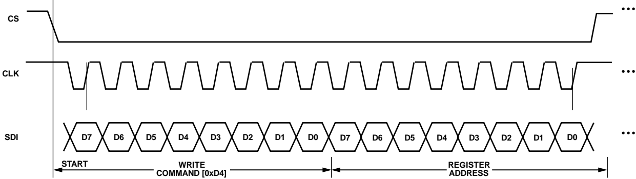
Figure 66. SPI Byte Write Example
