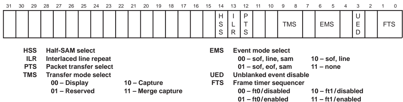
Figure 51. FMEMCTLx Register
