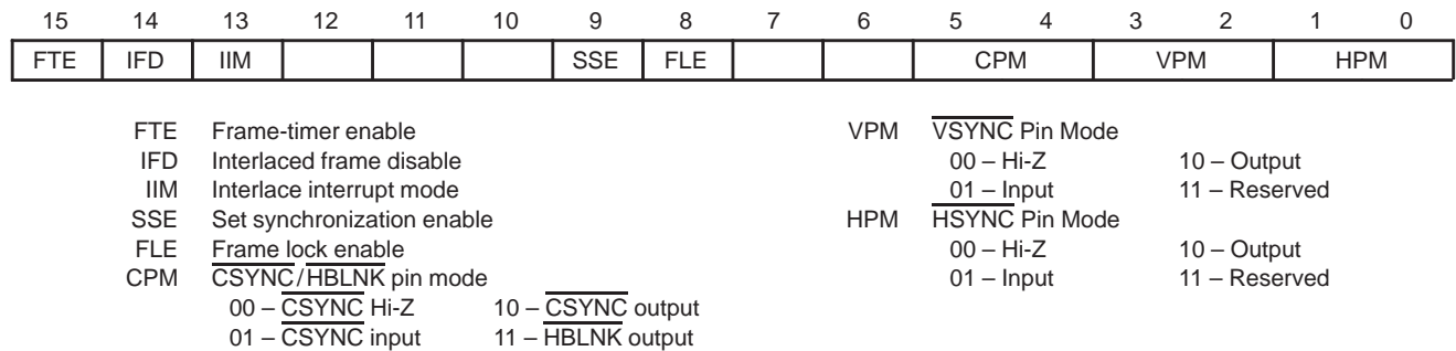
Figure 49. FTCTLx Register
