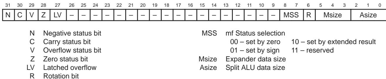
Figure 26. sr Format
