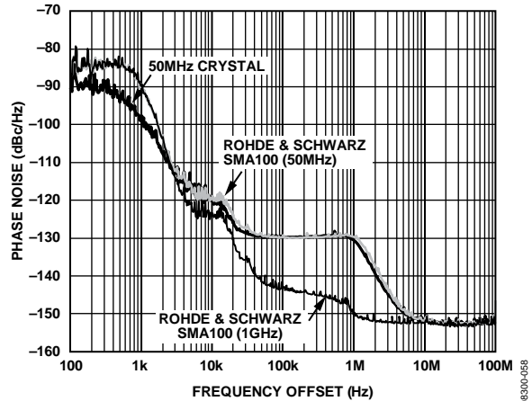
Figure 10. Absolute Phase Noise Comparison of SYSCLK Input Options (Output Driver = LVPECL), f_{REF} = 19.44 \text{ MHz} , f_o = 311.04 \text{ MHz} , LBW = 1 \text{ kHz}
