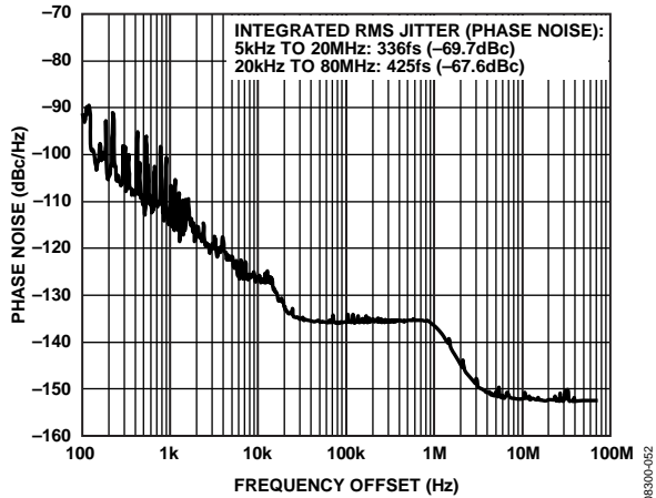
Figure 11. Absolute Phase Noise (Output Driver = LVPECL), f_{REF} = 8 \text{ kHz} , f_o = 155.52 \text{ MHz} , LBW = 100 \text{ Hz} , f_{SYSCLK} = 50 \text{ MHz} (Crystal), PLL On
