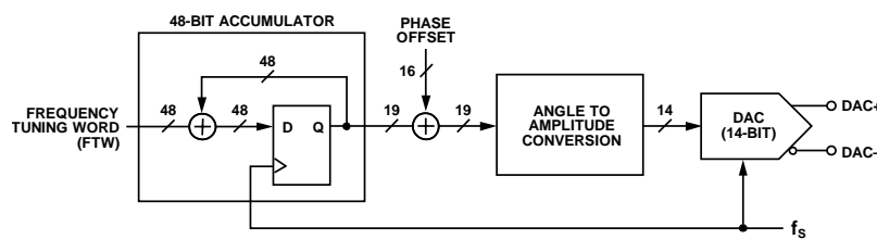
Figure 42. DDS Block Diagram
