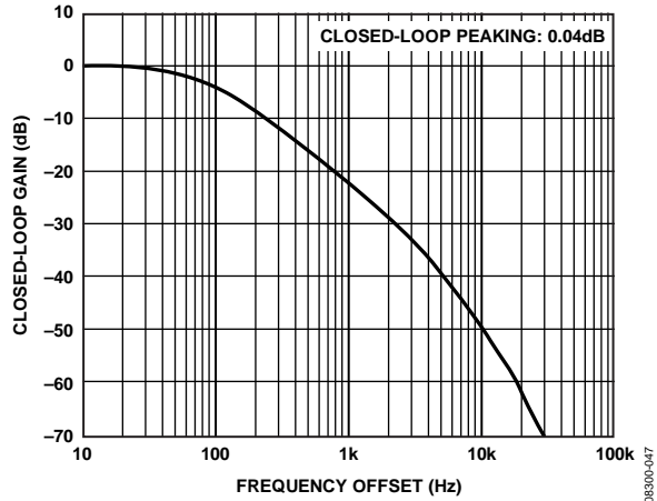
Figure 12. Jitter Transfer Bandwidth, Output Driver = LVPECL, f_{REF} = 19.44 \text{ MHz} , f_o = 155.52 \text{ MHz} , LBW = 100 \text{ Hz} (Phase Margin = 88°), f_{SYSCLK} = 1 \text{ GHz} , PLL Off
