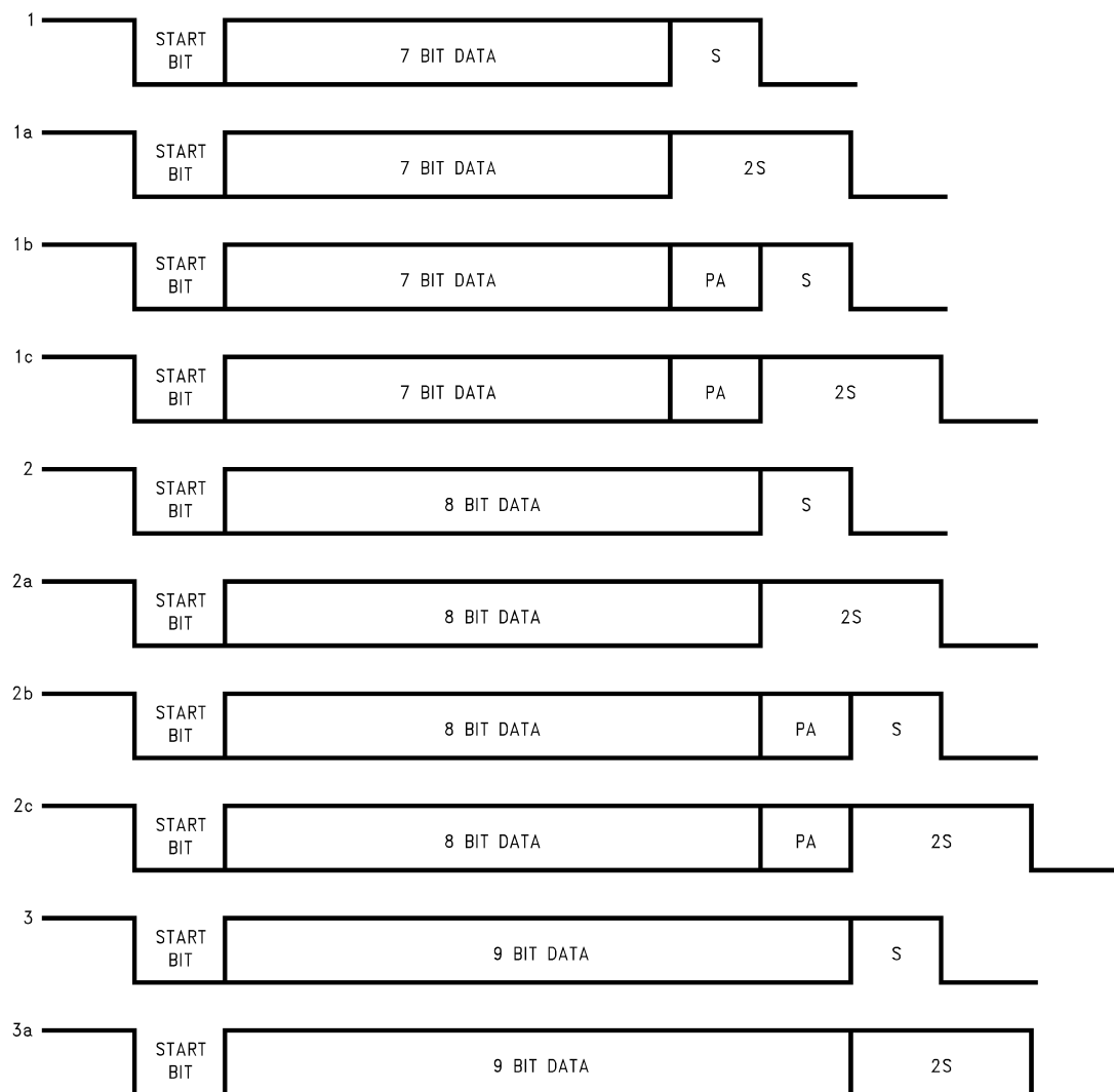
Figure 5-17. Framing Formats
