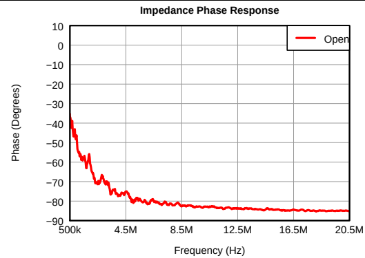
Figure 9. Input Impedance Without Active Termination (Phase)
