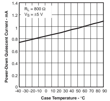
POWER-DOWN QUIESCENT CURRENT VS CASE TEMPERATURE
