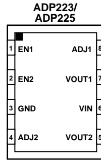
Figure 4. ADP223/ADP225 Pin Configuration
