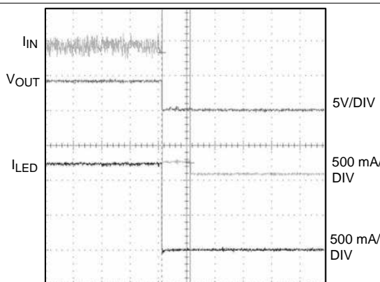
Figure 25. V_{OUT} Short Fault
