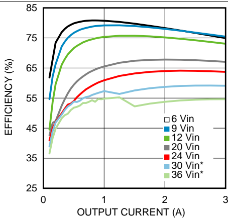
Figure 9. Efficiency 1.8-V Output at 25°C Ambient
