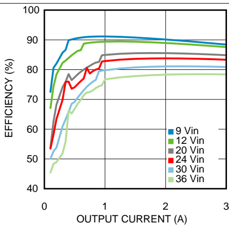
Figure 19. Efficiency 6-V Output at 85°C
