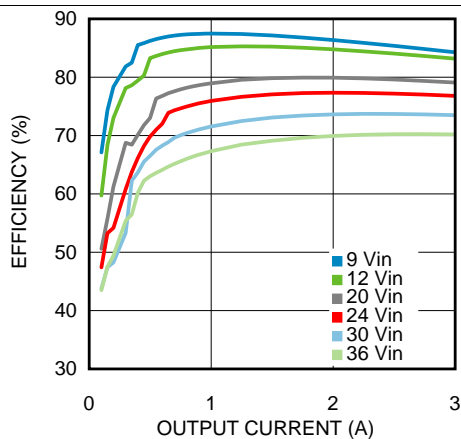
Figure 21. Efficiency 5-V Output at 85°C Ambient
