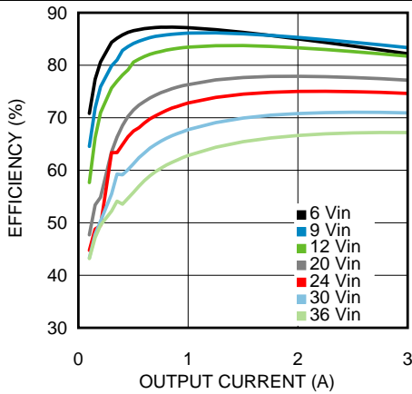
Figure 7. Efficiency 2.5-V Output at 25°C Ambient
