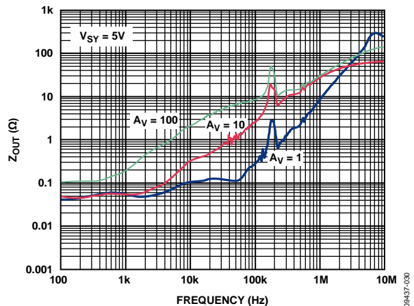
Figure 37. Closed-Loop Output Impedance vs. Frequency
