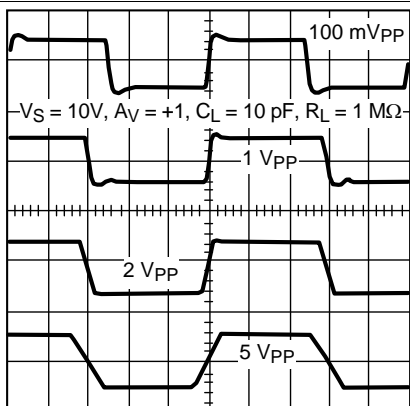
Figure 37. Step Response for Various Amplitudes
