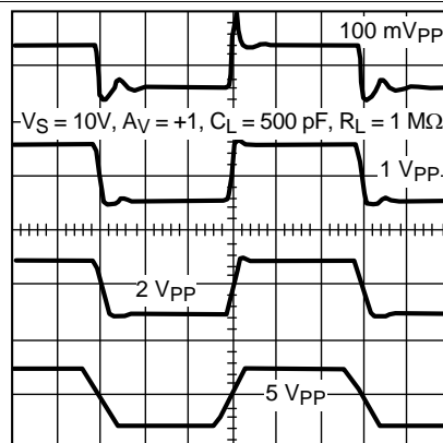
Figure 38. Step Response for Various Amplitudes
