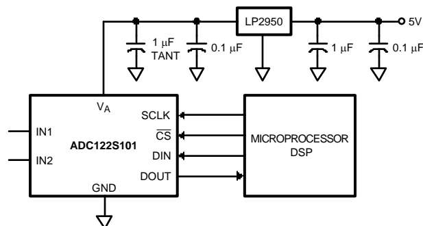
Figure 52. Typical Application Circuit
