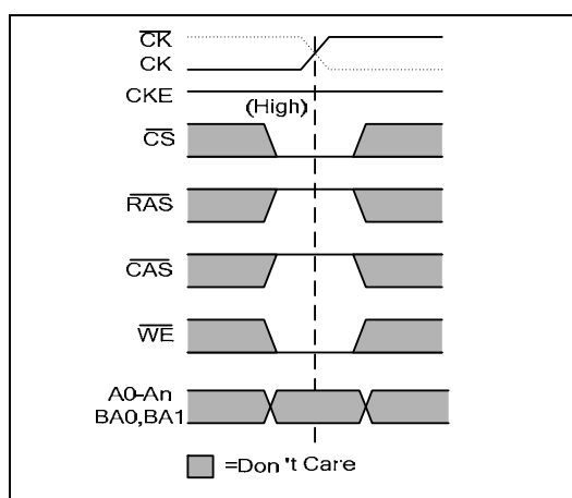
Figure 21 — Burst Terminate Command
