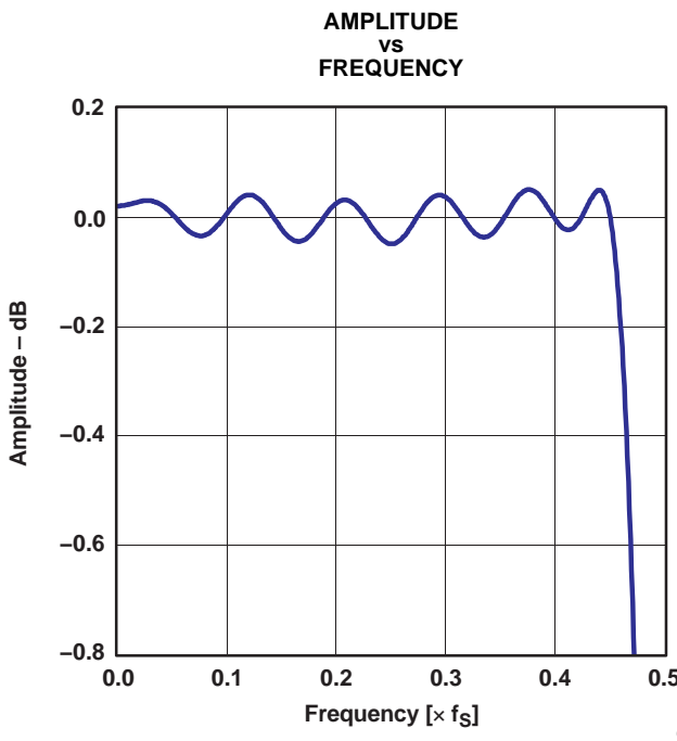
Figure 18. Pass-Band Ripple
