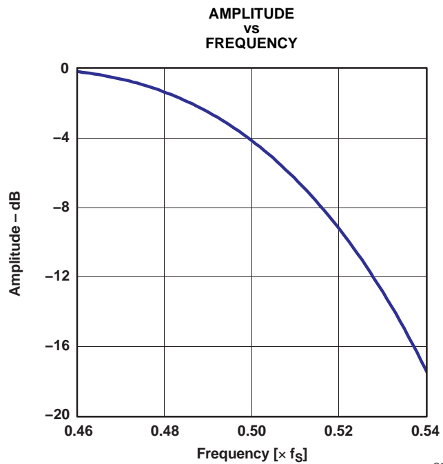
Figure 19. Transition-Band Response
