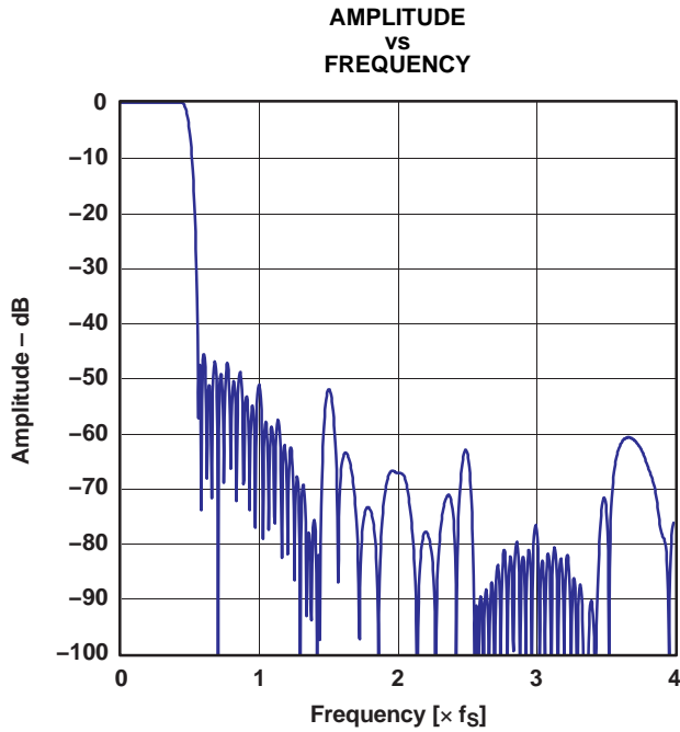
Figure 24. Stop-Band Attenuation
