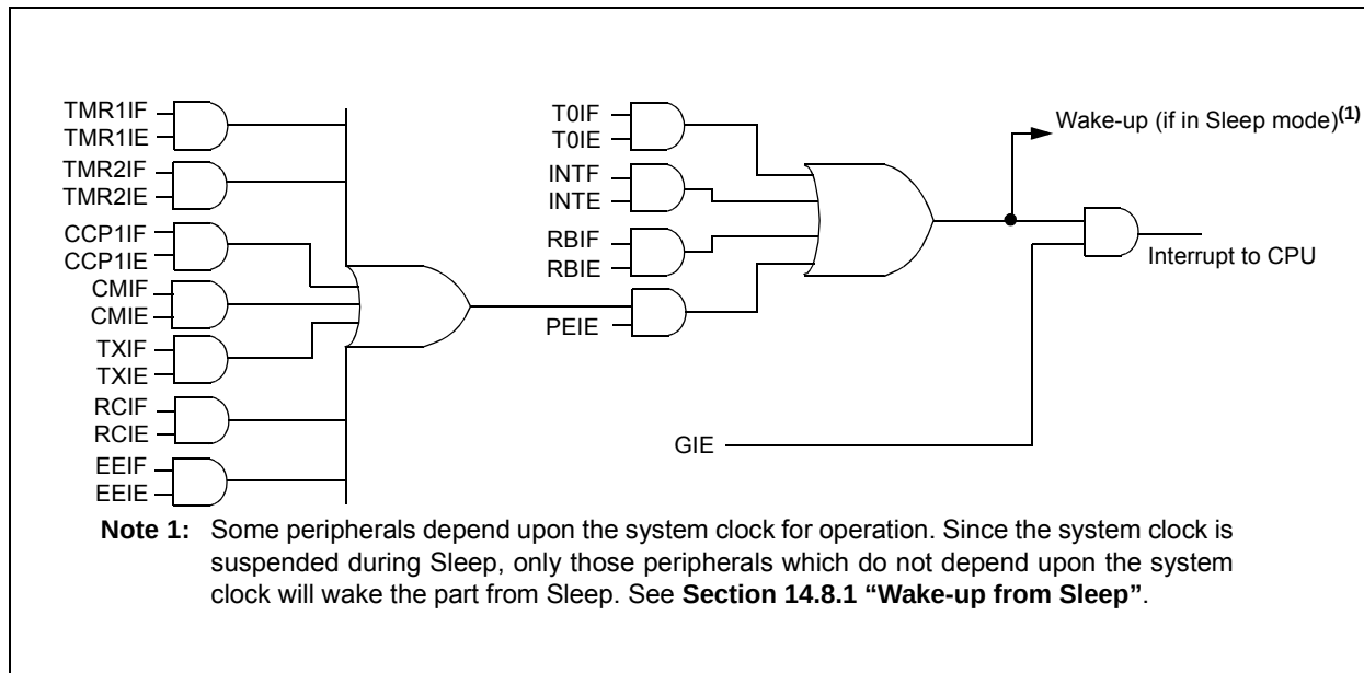
FIGURE 14-14: INTERRUPT LOGIC
