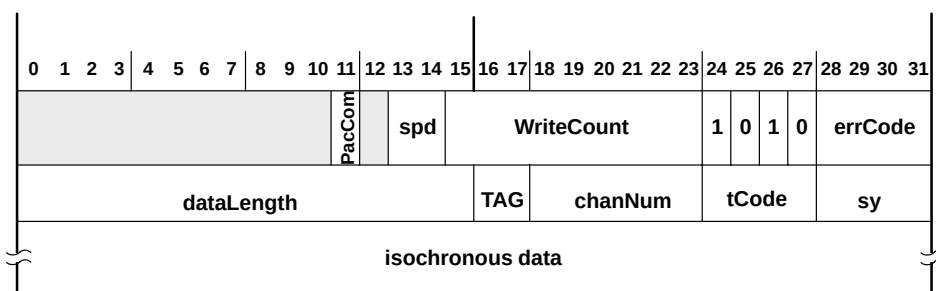
Figure 4–18. Isochronous-Receive Format
