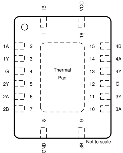
Not to scale Figure 5-2. RGY Package 16-Pin VQFN (Top View)
