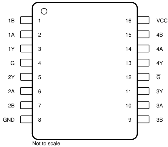
Not to scale Figure 5-1. D, NS, or PW Package, 16-Pin SOIC, SO, or TSSOP (Top View)
