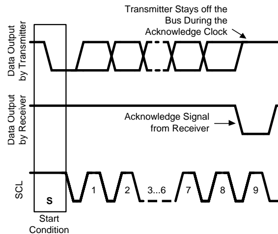
Figure 21. Acknowledge Signal
