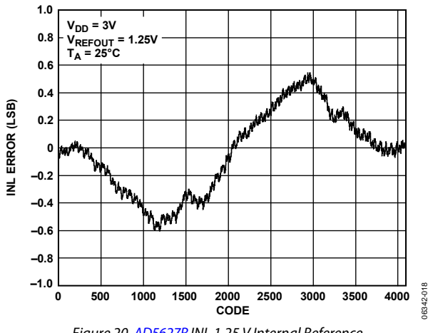
Figure 20. AD5627R INL, 1.25 V Internal Reference
