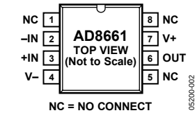
Figure 1. AD8661, 8-Lead SOIC_N (R-8)
