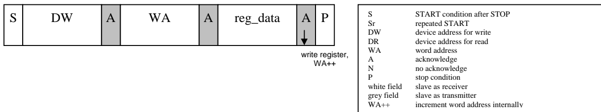
Figure 24 – PC Byte-Write:
