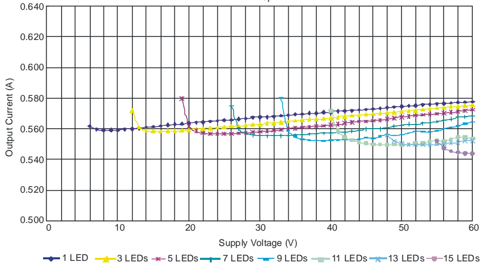
ZXLD1356Q Output Current Deviation (Normalized) L = 220μH
