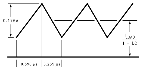
Figure 20. 10µH Inductor Current 5V - 12V Boost (LM4960)
