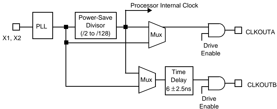
Figure 9. Clock Organization
