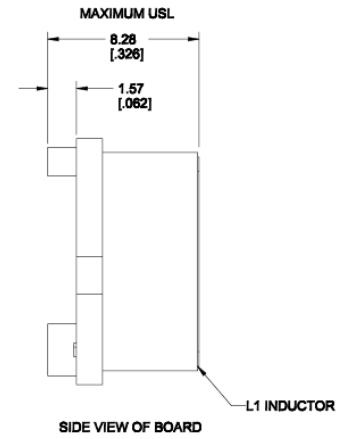
SIDE VIEW OF BOARD
