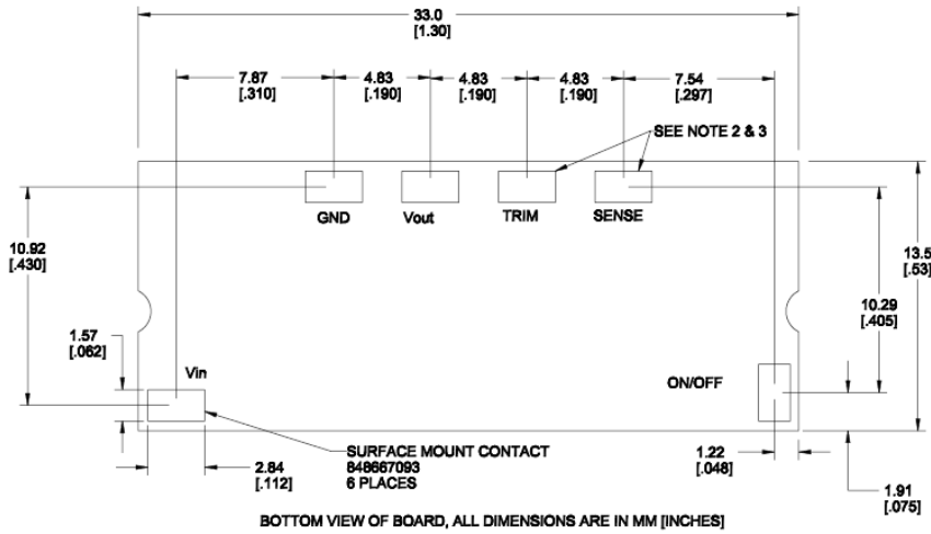
BOTTOM VIEW OF BOARD, ALL DIMENSIONS ARE IN MM [INCHES]
