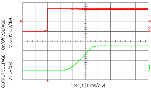
Figure 15. Typical Start-Up Using Remote On/Off with Low-ESR external capacitors ( C_o = 5000\ \mu\text{F} ) ( V_{in} = 12.0\text{ Vdc} , V_o = 5.0\text{ Vdc} , I_o = 10.0\text{ A} , C_o = 1050\ \mu\text{F} ).
