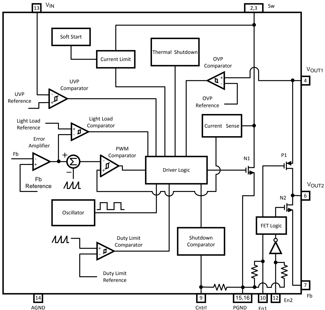
Figure 4. Block Diagram
