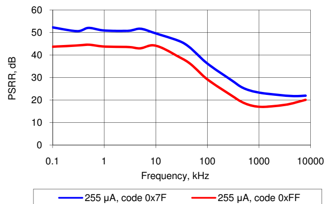
Figure 11-46. IDAC PSRR vs Frequency
