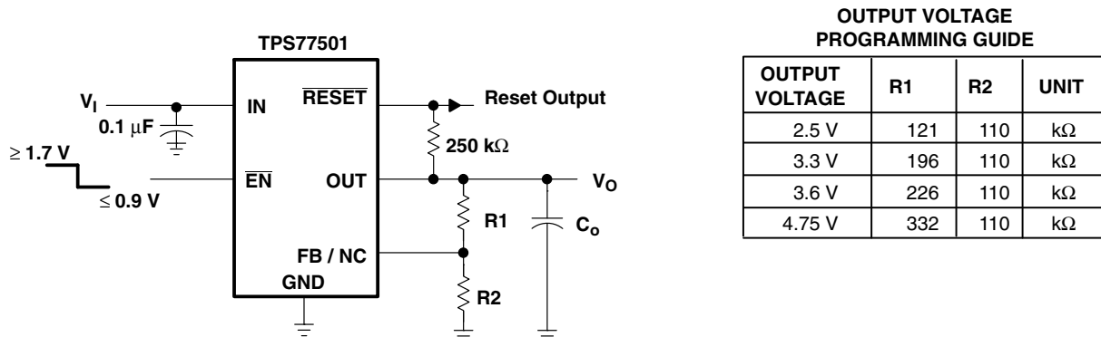
Figure 26. TPS77501 Adjustable LDO Regulator Programming
