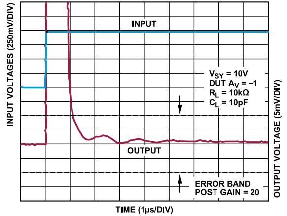
Figure 77. Positive Settling Time to 0.1%, V_{SY} = 10\text{ V}
