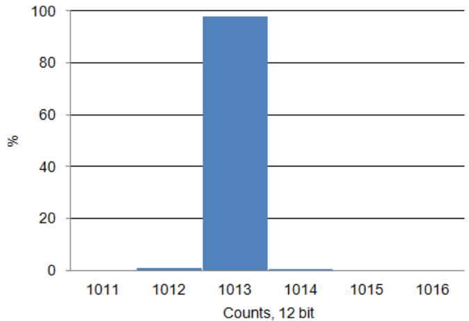
Figure 11-30. SAR ADC Noise Histogram, 1000 samples, 700 kps, Internal Reference Bypassed, V_{IN} = V_{REF}/2
