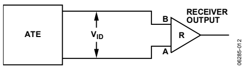
Figure 12. Receiver Propagation Delay Test Circuit
