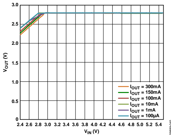
Figure 35. LDO Line Regulation Across Output Load, VOUT3 = 2.8 V
