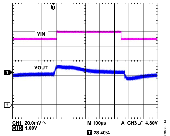
Figure 38. LDO Response to Line Transient, VIN = 4.5 V to 5 V, VOUT3 = 2.8 V
