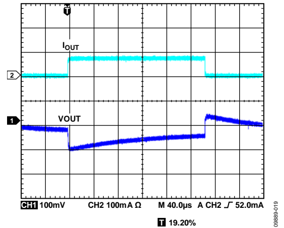
Figure 37. LDO Response to Load Transient, IOUT3 = 1 mA to 80 mA, VOUT3 = 2.8 V
