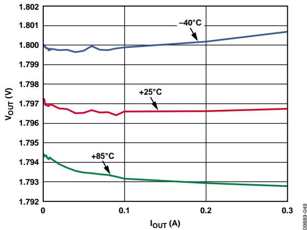
Figure 34. LDO Load Regulation Across Temperature, VIN3 = 3.6 V, VOUT3 = 1.8 V
