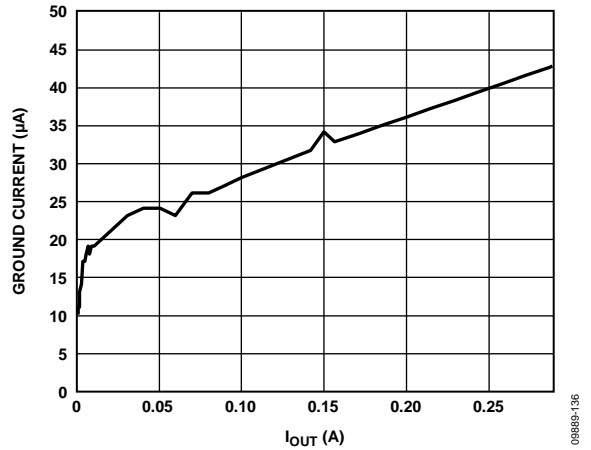
Figure 36. LDO Ground Current vs. Output Load, VIN3 = 3.3 V, VOUT3 = 2.8 V
