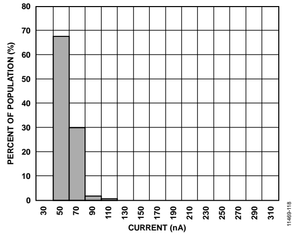
Figure 12. Standby Mode Current Consumption, V_S = V_{DDI/O} = 3.3 V , 25°C
