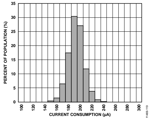
Figure 13. Current Consumption, Measurement Mode, Data Rate = 100 Hz, V_S = V_{DDI/O} = 3.3 V , 25°C
