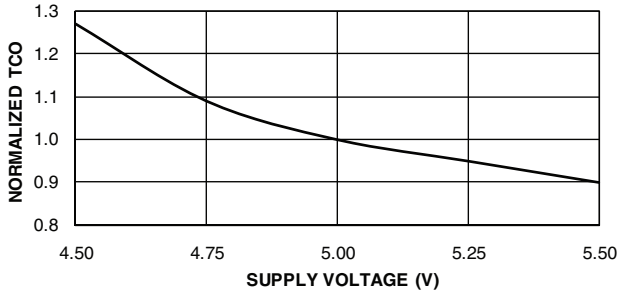
ATMEL ATF22V10C/CQ NORMALIZED T_{CO} VS. V_{CC}
