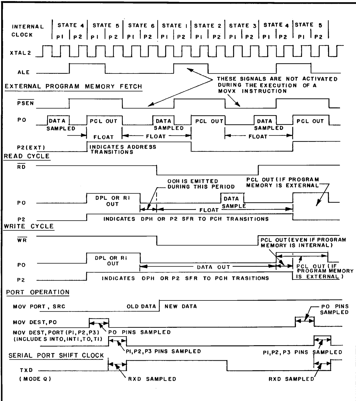
FIGURE 4. Clock waveforms.
