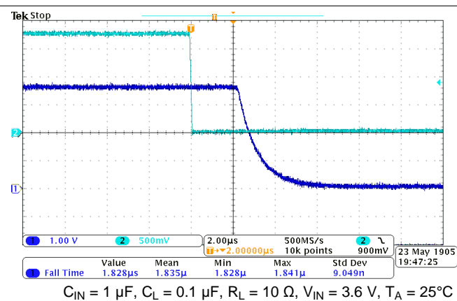
Figure 21. Turn-Off Response
