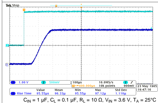
Figure 20. Turn-On Response
