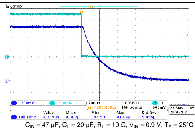
Figure 19. Turn-Off Response
