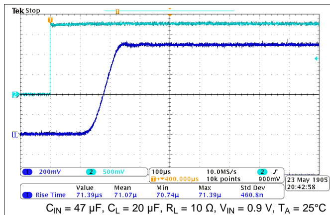
Figure 18. Turn-On Response
