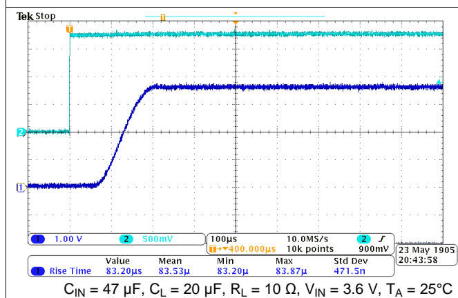
Figure 22. Turn-On Response
