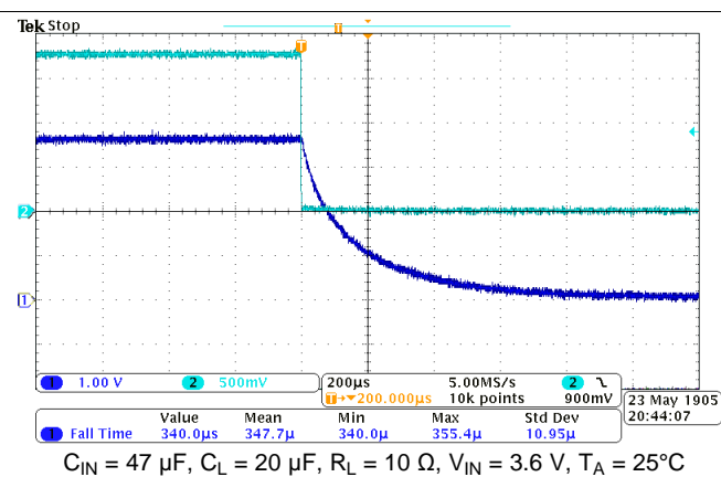
Figure 23. Turn-Off Response
