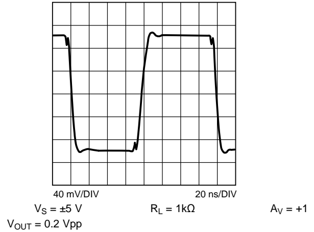
Figure 38. Small Signal Step Response
