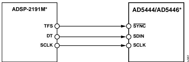
Figure 46. ADSP-2191M to AD5444/AD5446 Interface
