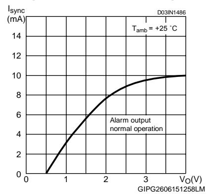
Figure 11: Current sourcing
