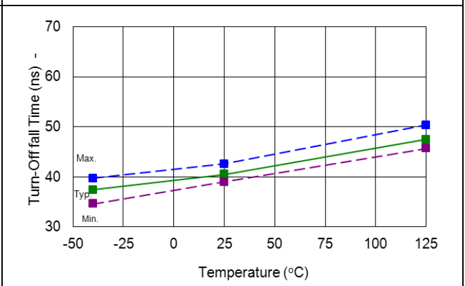
Figure 41. Turn-off fall time vs. temperature
