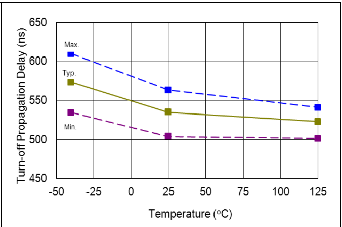
Figure 39. Turn-off propagation delay vs. temperature
