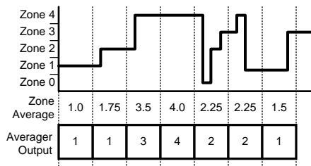
Figure 28. Averager Calculation
