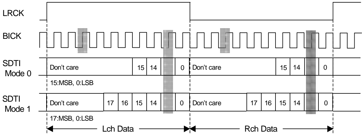
Figure 4. Mode 0,1 Timing
