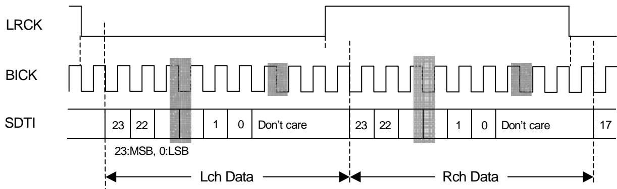
Figure 6. Mode 3 Timing
