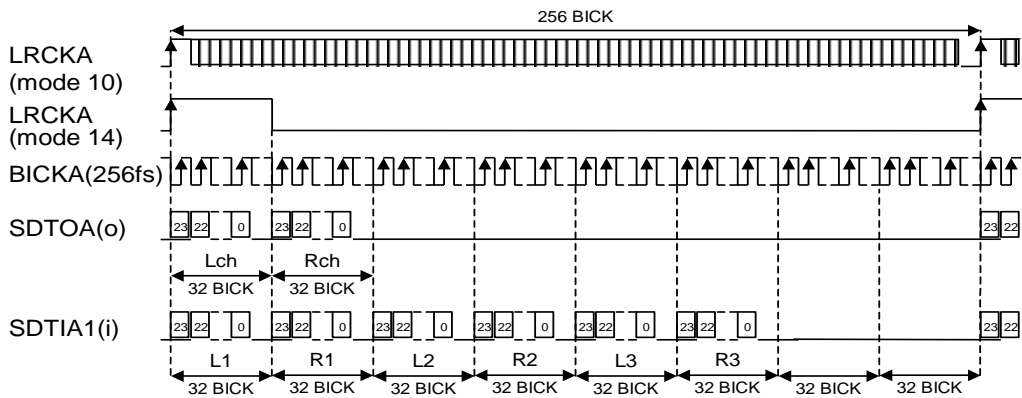
Figure 14. Mode 10 ,14 Timing
