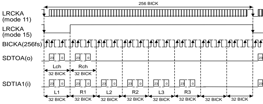
Figure 15. Mode 11 ,15 Timing
