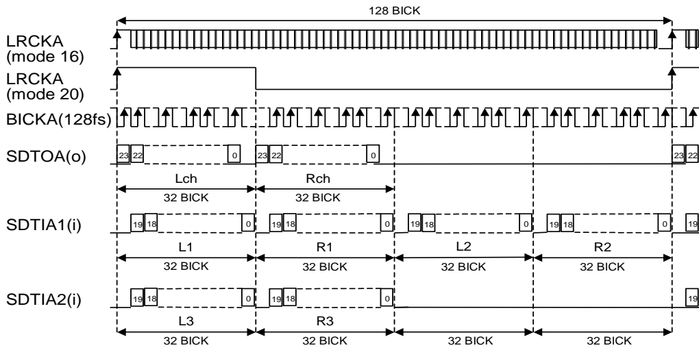
Figure 16. Mode 16 ,20 Timing
