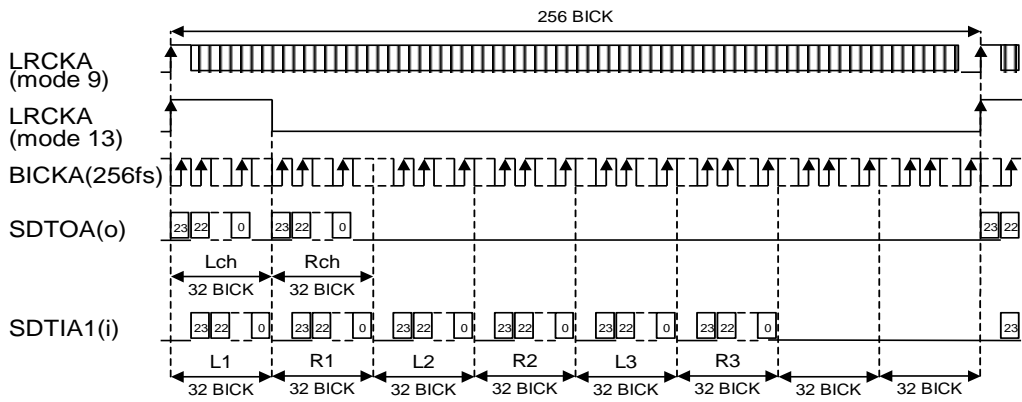
Figure 13. Mode 9 ,13 Timing
