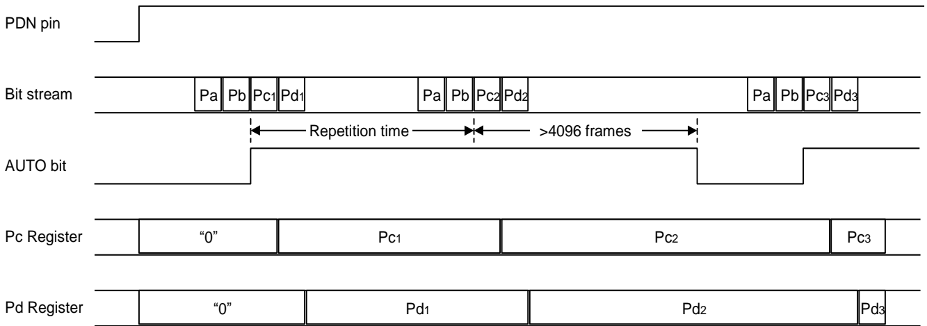
Figure 38. Timing example 1
