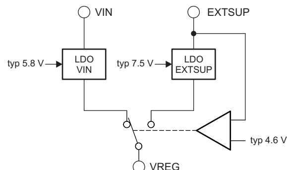
Figure 20. Internal Gate-Driver Supply
