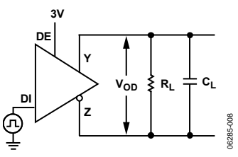
Figure 8. Driver Timing Test Circuit
