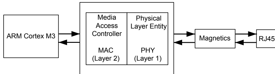
Figure 19-1. Ethernet Controller
