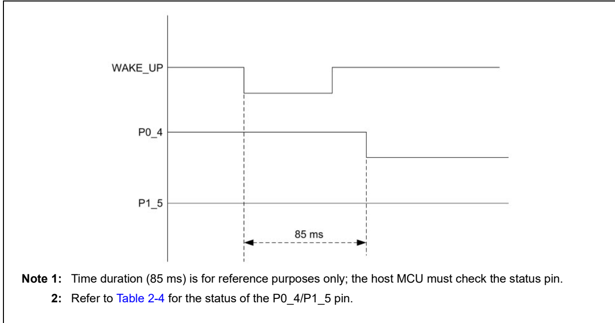
FIGURE 2-5: WAKE-UP TIME
