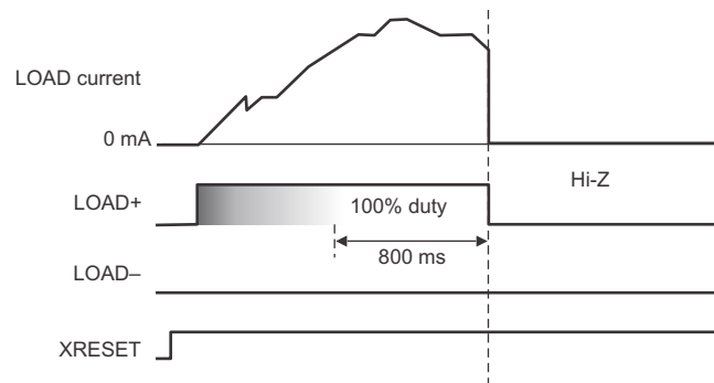
Figure 7. Overcurrent Protection Load 1-Channel
