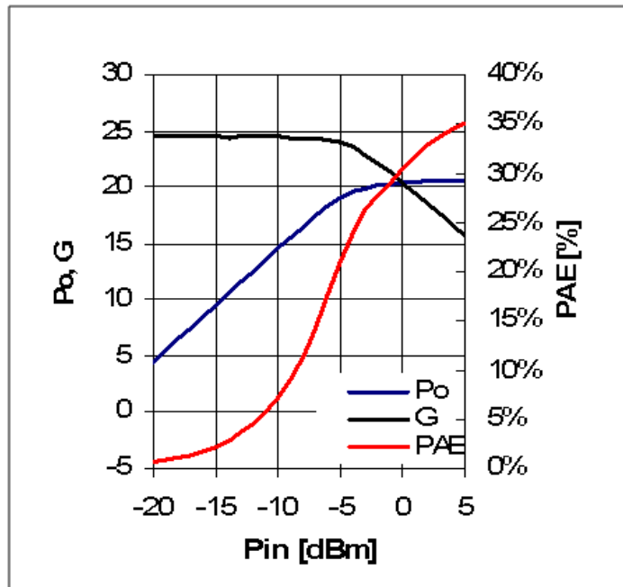
Pin-Pout-Gain
